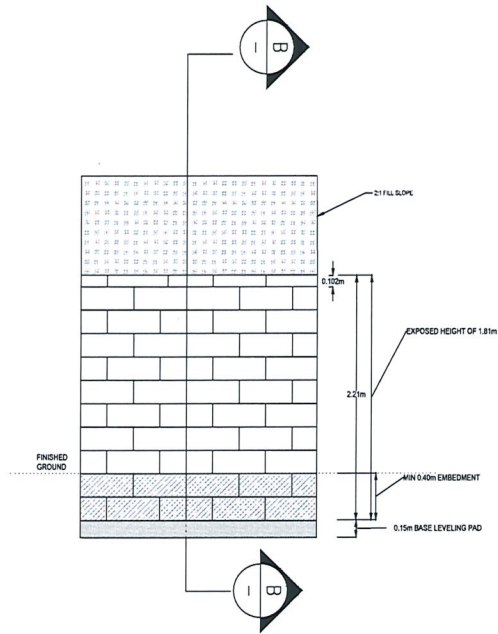
FRONT SECTION - MAXIMUM HEIGHT AT 2:1 FILL SECTION
