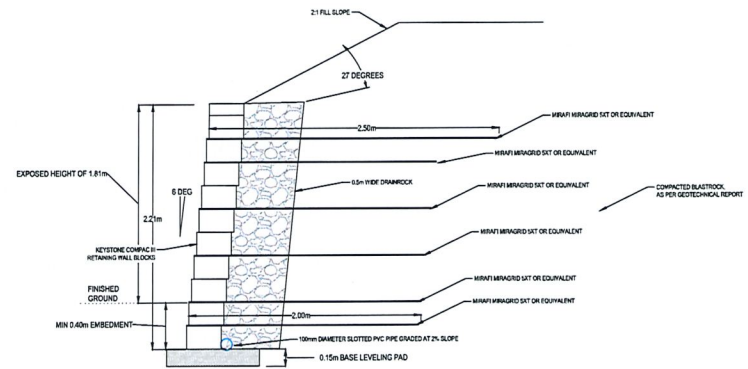
CROSS SECTION - MAXIMUM HEIGHT AT 2:1 FILL SECTION
